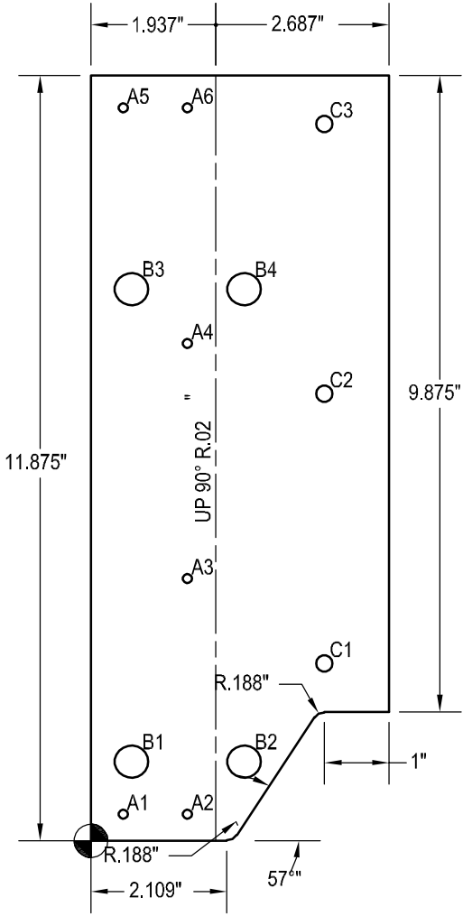
PART 1 FLAT PATTERN SCALE 3/8" = 1"
