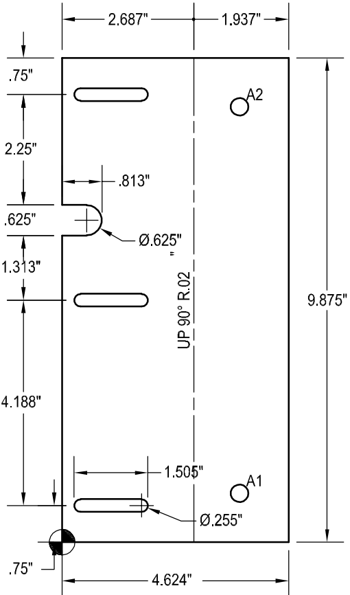
PART 2 FLAT PATTERN SCALE 3/8" = 1"
